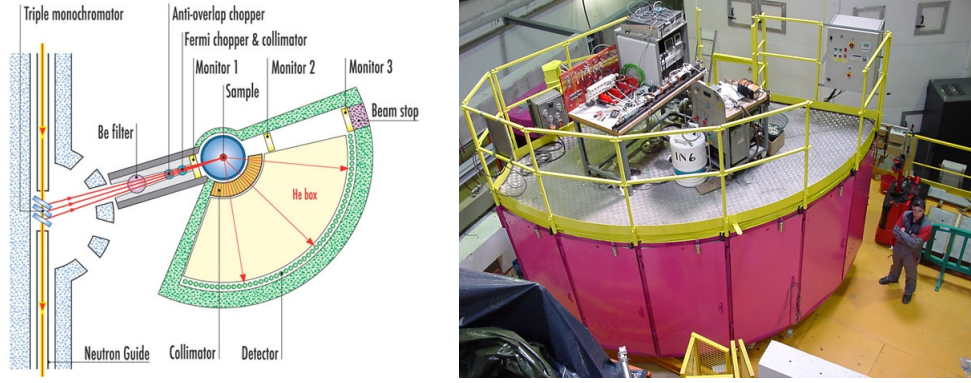
Figure 1.20: Time of Flight (TOF) spectrometer IN6-ILL (Grenoble, France)
