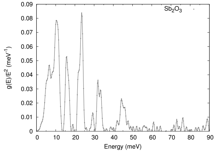
Figure A.2: Density of phonon states of \text{Sb}_2\text{O}_3 [1]
