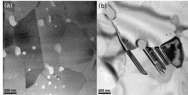
Figure 4.2: (a) TEM image of \text{SiGe} sample showing large grains (dark) and amorphous spherical precipitates (light). (b) TEM bright-field image showing defects as twins on a nanocrystal and amorphous spherical precipitates.
