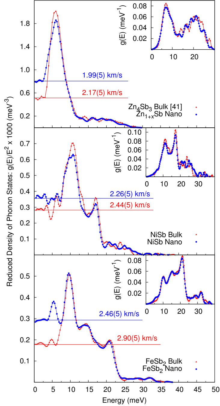
Figure 5.2: Reduced density of ^{121}\text{Sb} phonon states of nano \text{Zn}_{1+x}\text{Sb} , NiSb and FeSb 2 compared to the bulk counterpart: a decrease on the speed of sound is observed upon nanostructuration.
