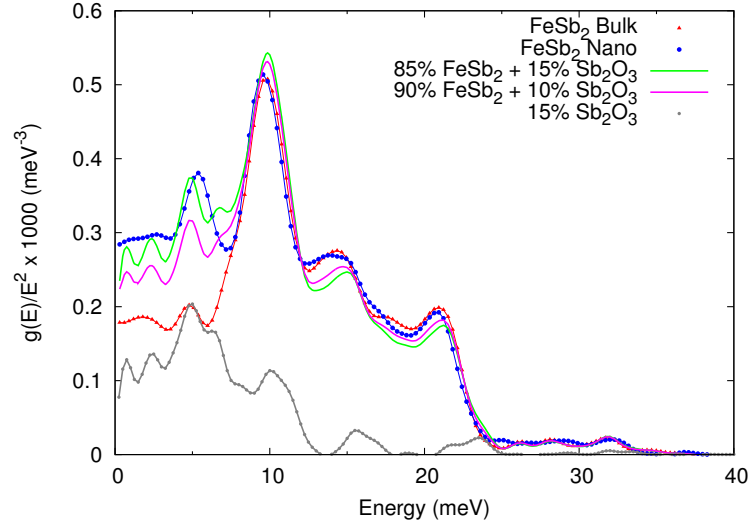
Figure A.1: Reduced density of phonon states of nano and bulk \text{FeSb}_2 , \text{Sb}_2\text{O}_3 and sums of bulk \text{FeSb}_2 with \text{Sb}_2\text{O}_3 : 85 + 15% and 90 + 10%.
