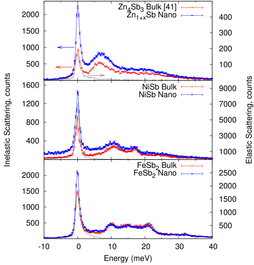
Figure 5.1: NIS spectra of nano \text{Zn}_{1+x}\text{Sb} , \text{NiSb} and \text{FeSb}_2 (blue circles) compared to the spectra of the bulk counterpart (red triangles). The elastic scattering is shown as gray line with y scale on the right side of the plots.
